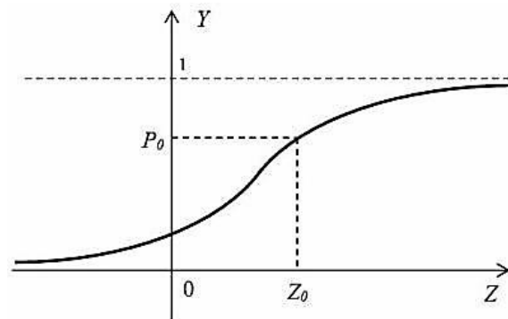
Figure 1. The binary logistic regression model
