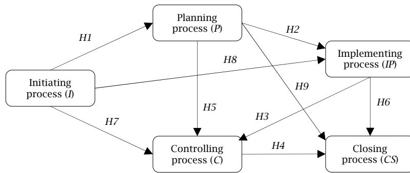
Figure 1. Hypothesis structure model
