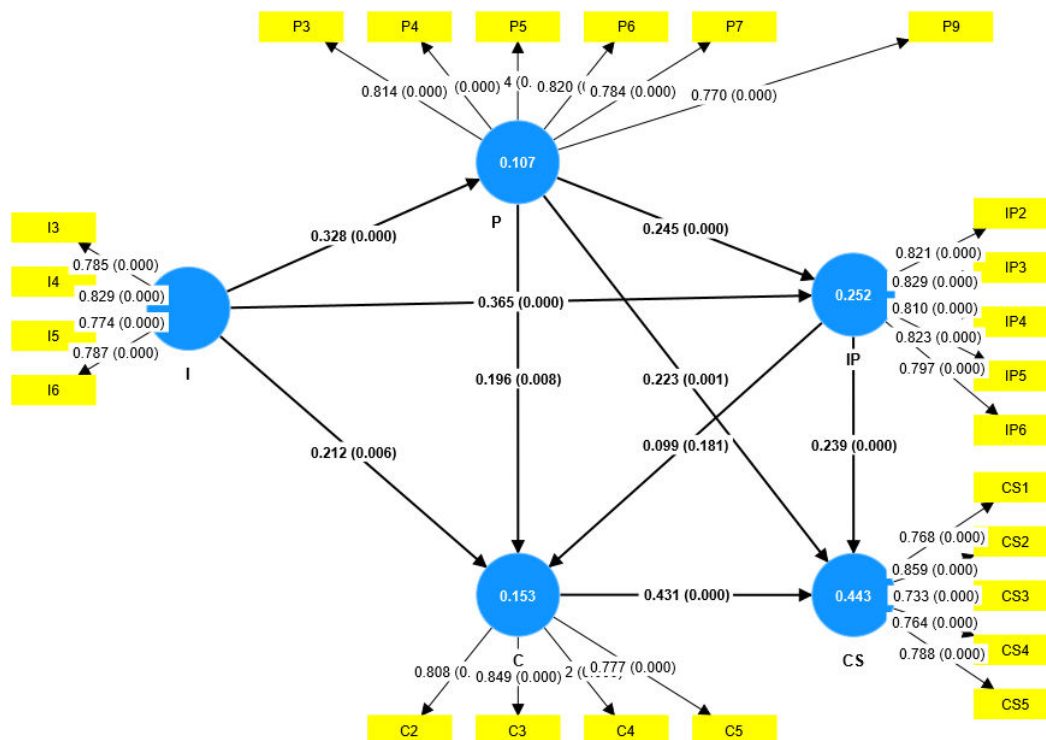
Figure 2. Model test results with no intermediate variables
